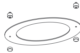
27.250 Colour ring blue Can be used in all elliptics versions
